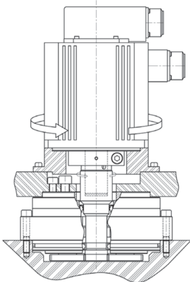
PQ-C3 바닥설치 (로봇기저축) [PQ-C3 floor mounting (Robot Swing axis)]
